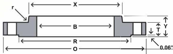
INDUSTRY STANDARD CLASS 300 SERIES "A" SLIP-ON FLANGES (BOLTING MATCHES)
