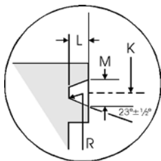
Ring joint facing dimensions - ASME/ANSI B16.5 and B16.47 Series A (MSS SP-44) and Series B (API 605) (Continued)
