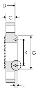
Ring joint facing dimensions - ASME/ANSI B16.5 and B16.47 Series A (MSS SP-44) and Series B (API 605) (Continued)
